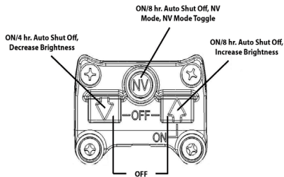
Fig 4: Pushbutton interface
